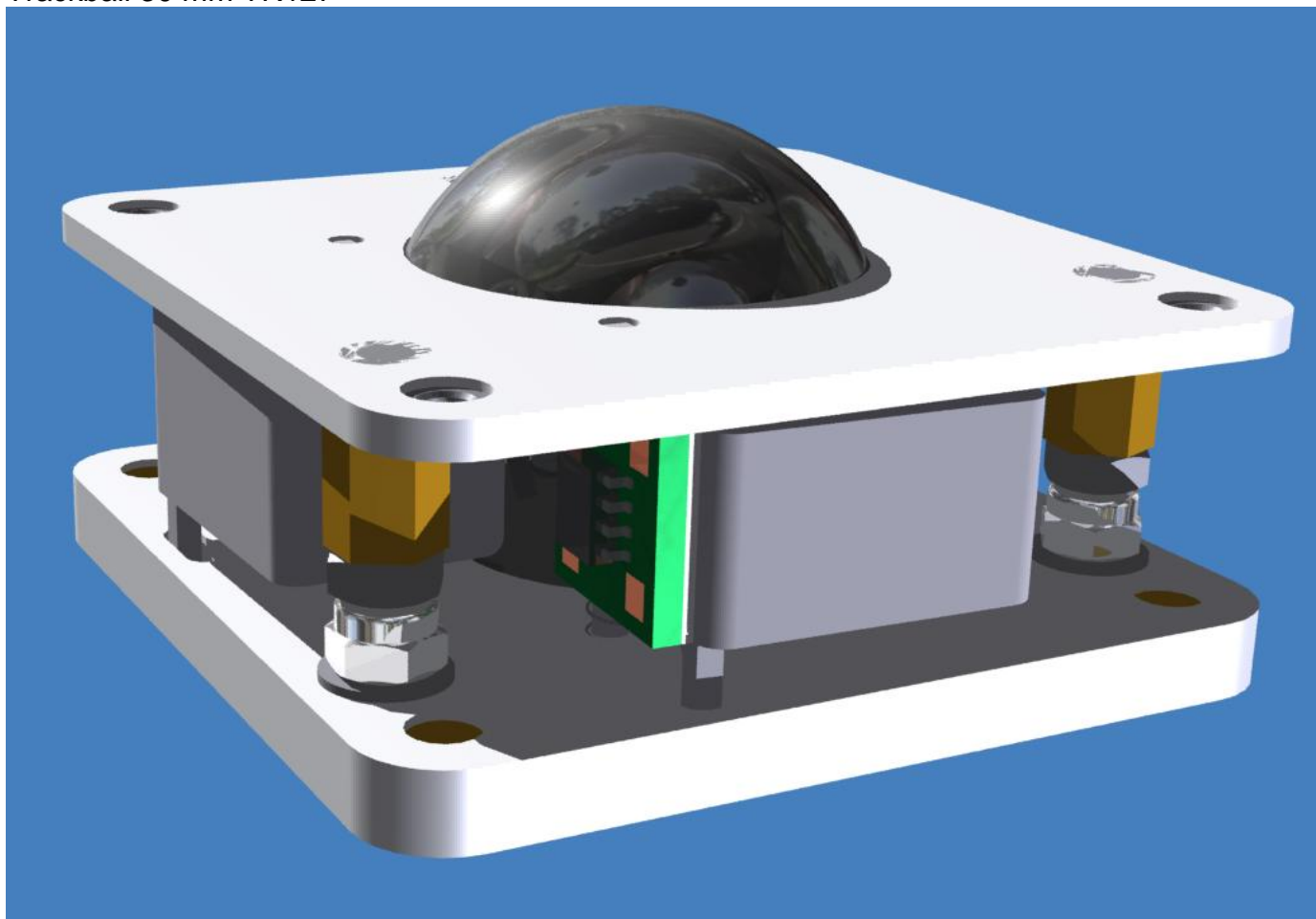
Trackball 30 mm TR127
